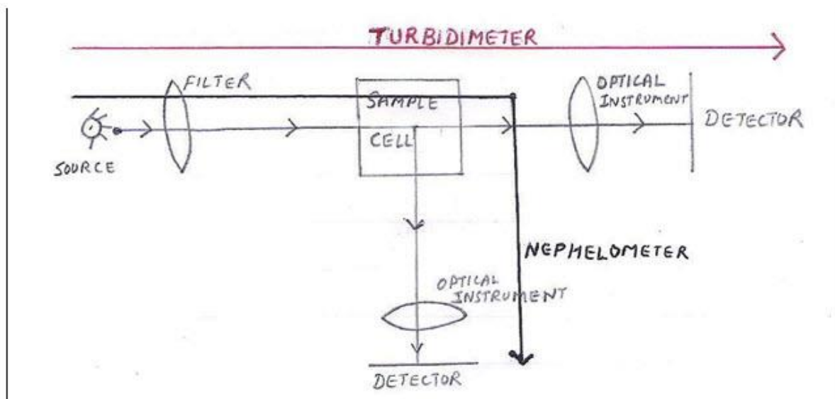
Figure 01: Components of Turbidimeter (straight line) & Nephelometer (line bent at right angle)
