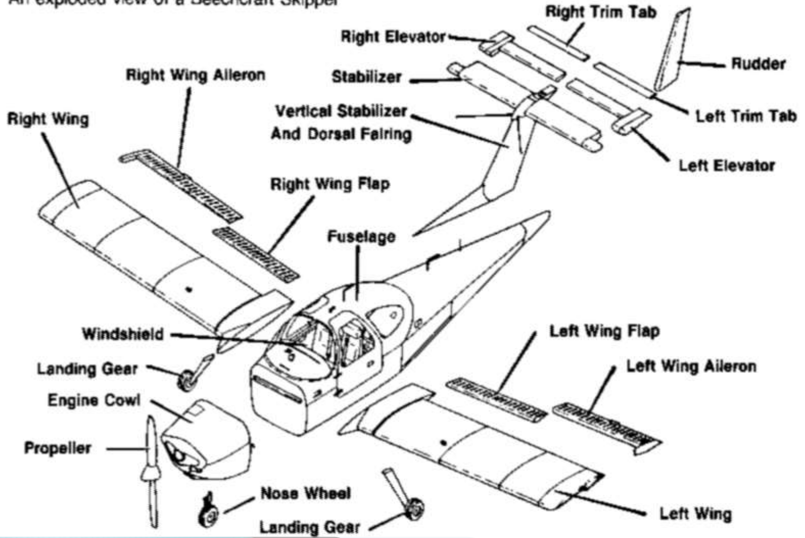
An exploded view of a Beechcraft Skipper
