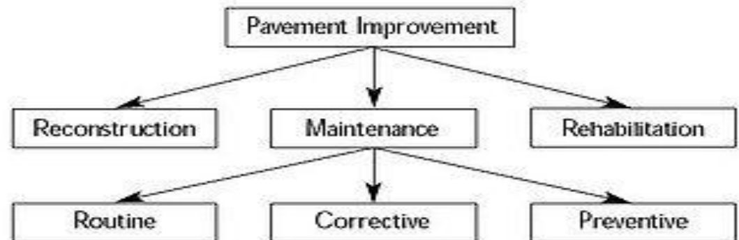
Hierarchical Model
