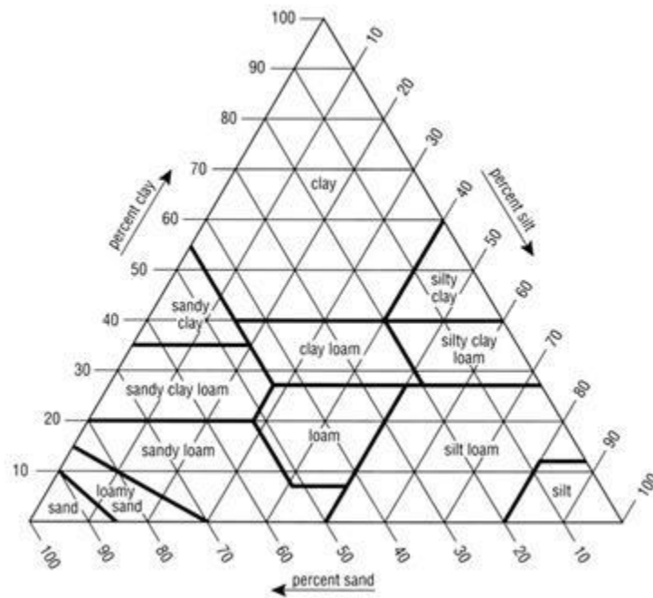
Range of soil separates in different textural classes:
