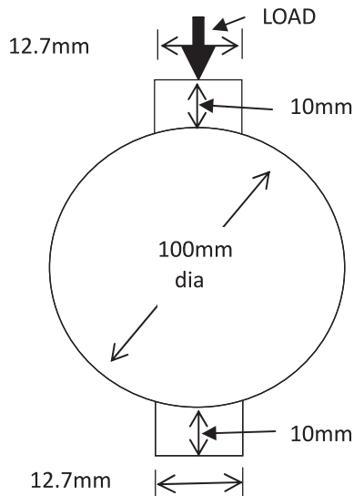
Fig. IX-II Marshall Samples of RAP 100 mm Diameter and 63 mm Long Under Indirect Tensile Test
