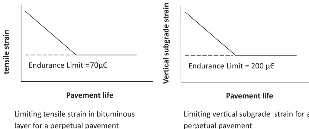
Fig. II-3 Limiting Design Strain for a Perpetual Pavement
