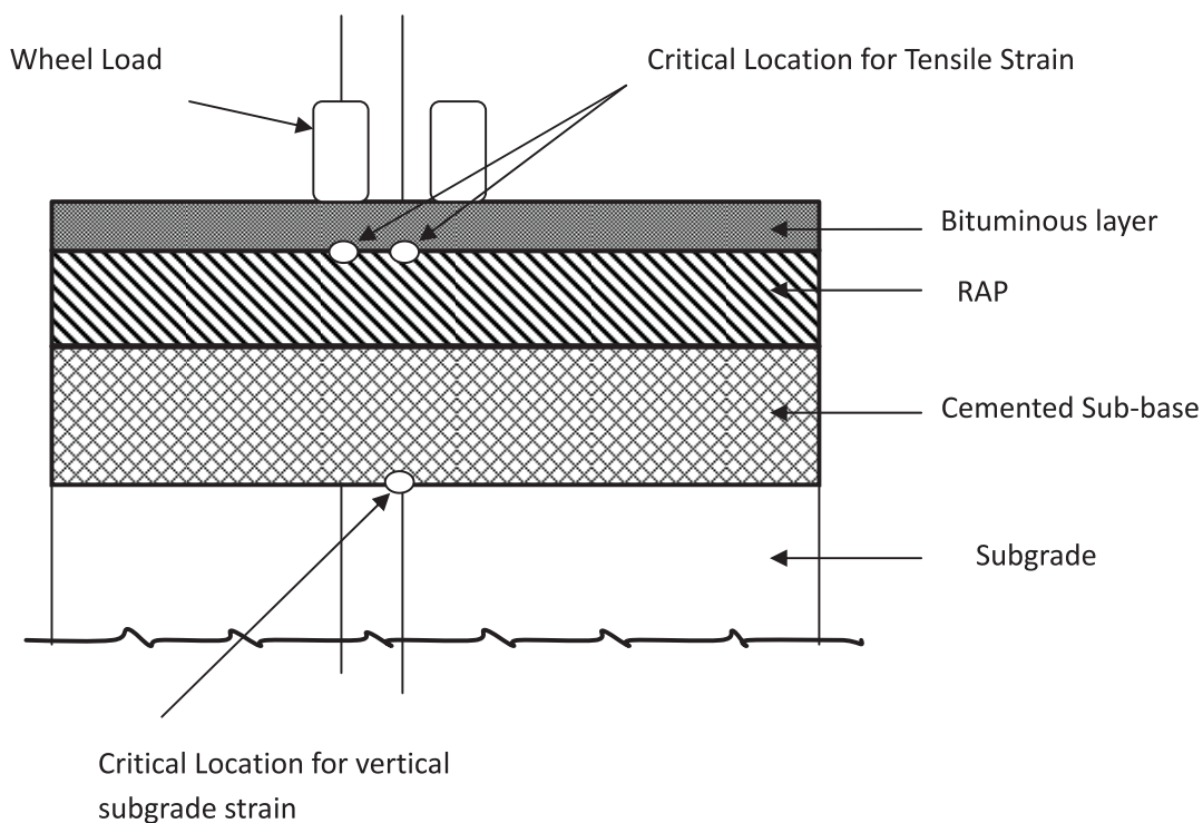
Fig. 10.4 Bituminous Surfacing with RAP and Cemented Sub-base
