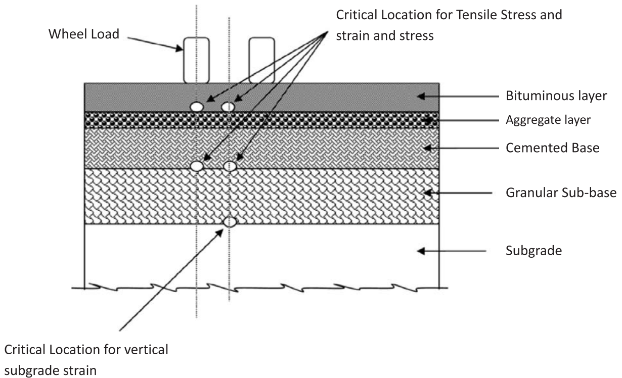
Fig. 10.5 Bituminous Surfacing, Cement Treated Base and Granular Sub-base with Aggregate Interlayer
