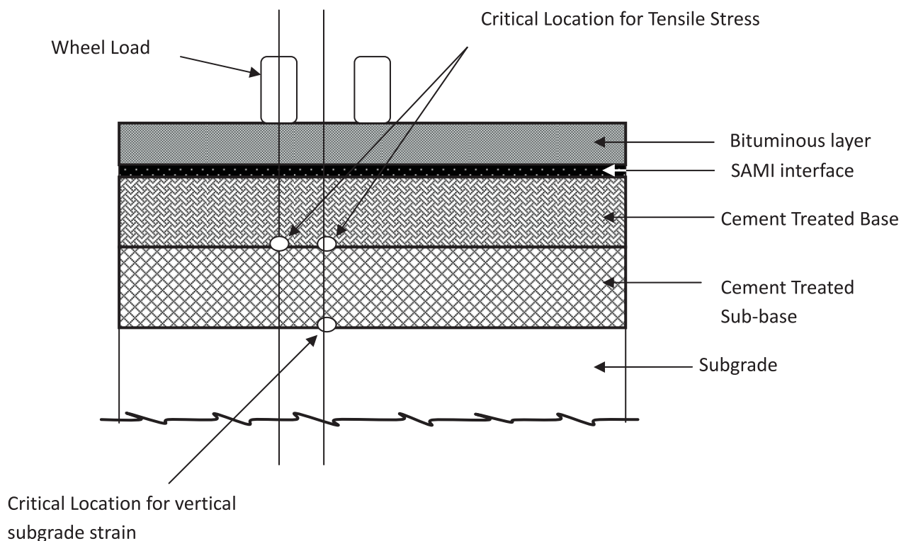
Fig. 10.3 Bituminous Surfacing with Cemented Granular Base and Cemented Granular Sub-base with Stress Absorbing Membrane Interlayer (SAMI)
