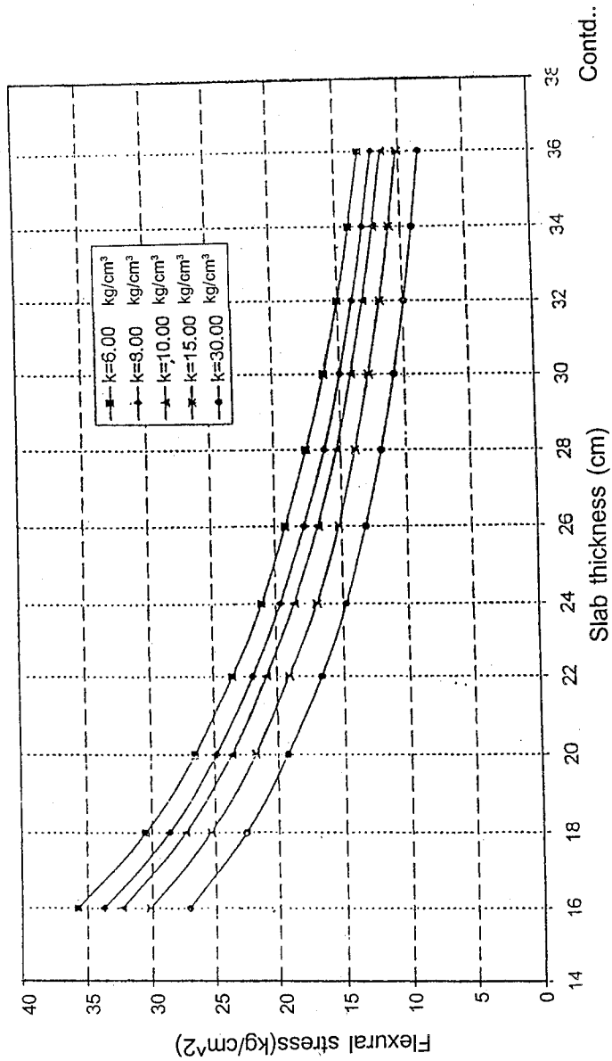
Stresses in Rigid Pavement (Tandem Axle Load 28 tons)
