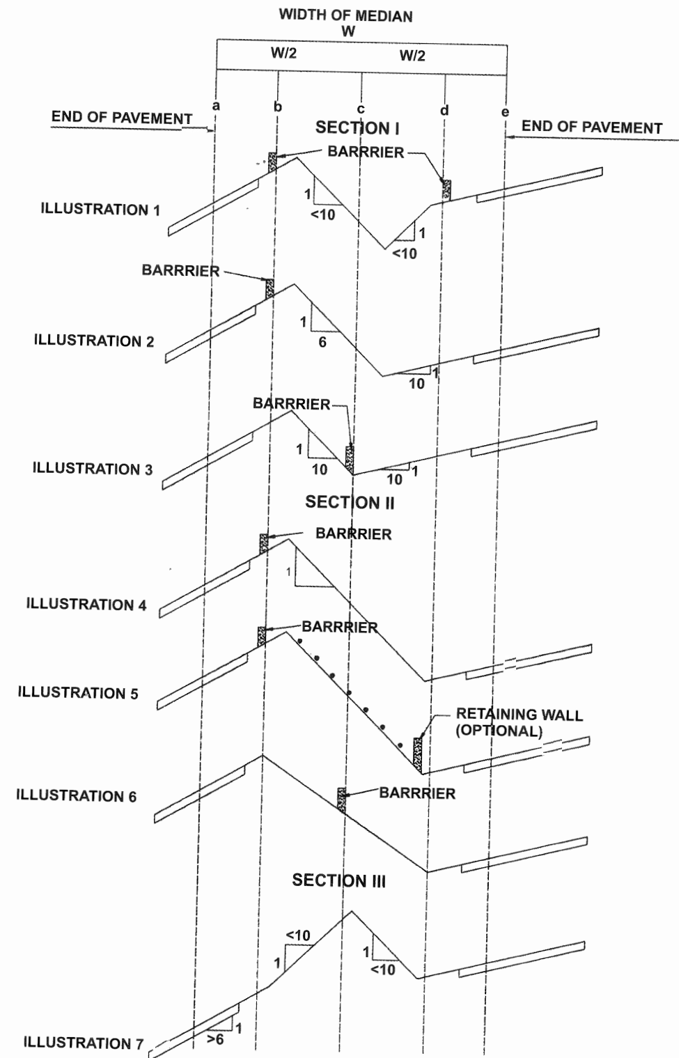
Fig. 9.10 Recommended Median Barrier Placement in Non-level Median
