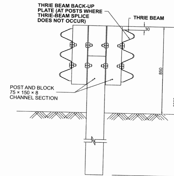
Fig. 9.9 Typical Details of Thrie Beam Median Barrier
