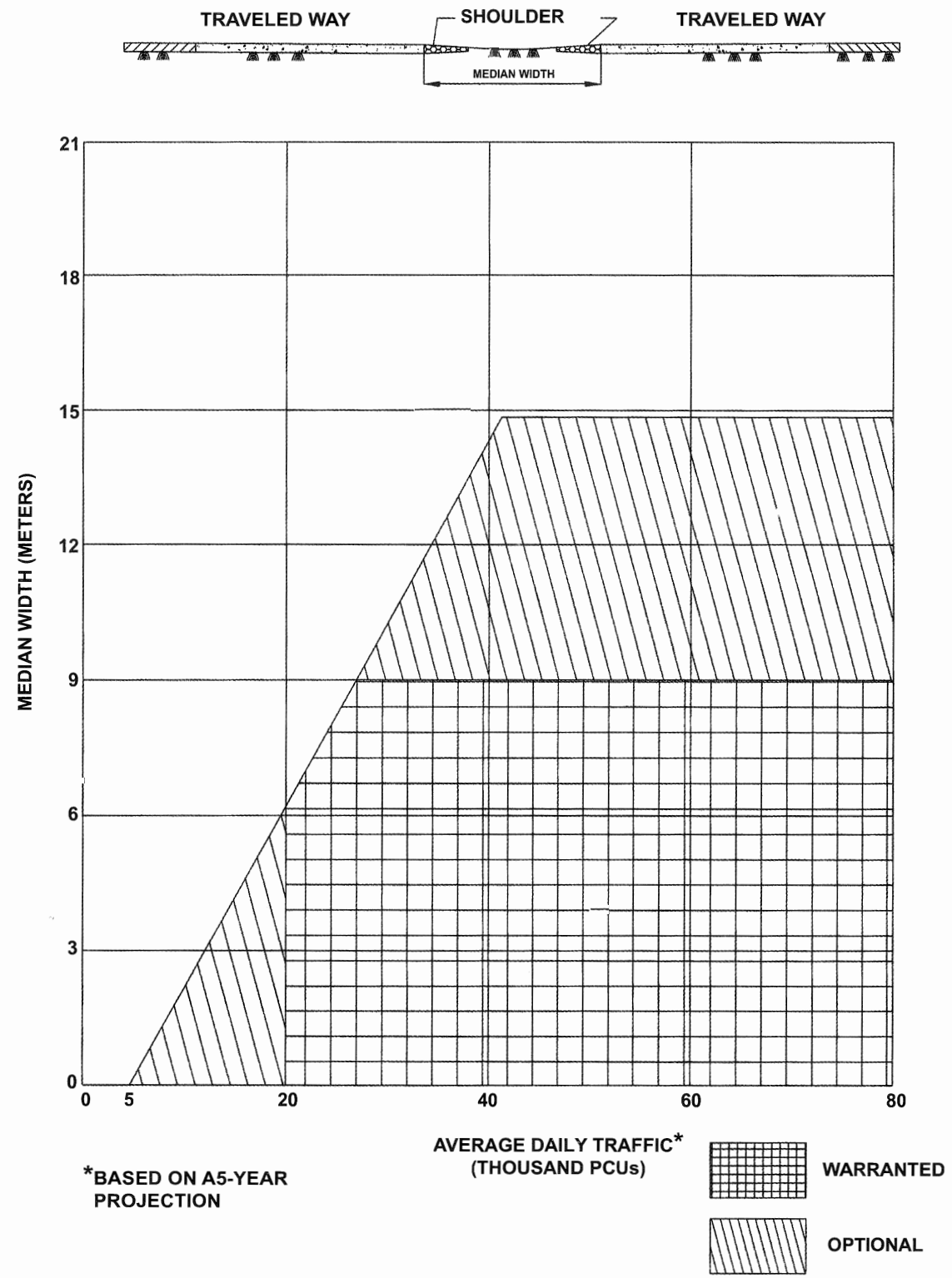
Fig. 9.7 Median Barrier Warrants
