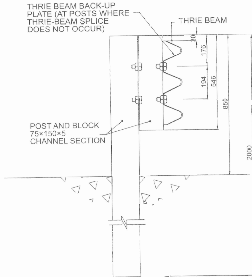
Fig. 9.3 Typical Details of Thrie Beam Section
