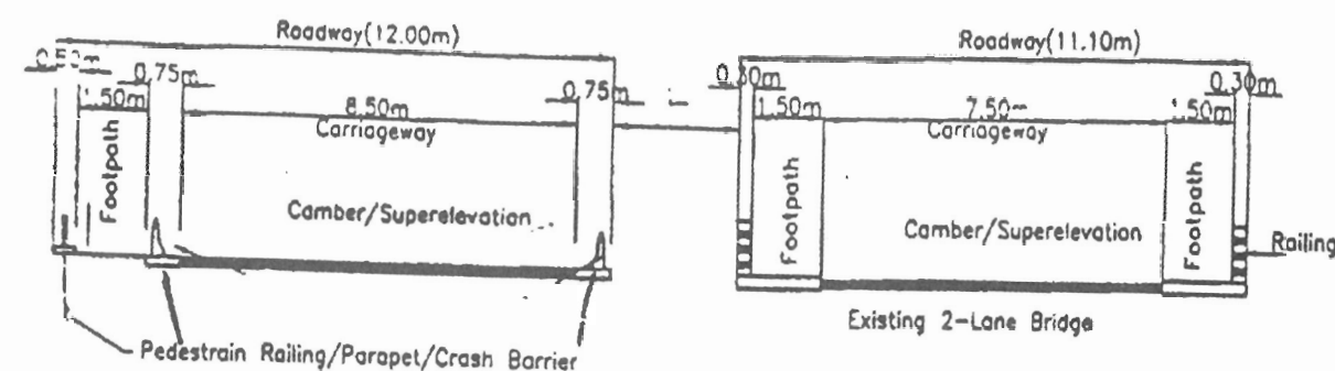
Fig. 7.4A Cross Section of Bridge at Deck Level - With Footpath (T-Beam/Box Girder Type / Well / Pile Foundation) 4-Lane Divided Highway (One side new Bridge and other sides Existing for 2-Lane Bridge)
