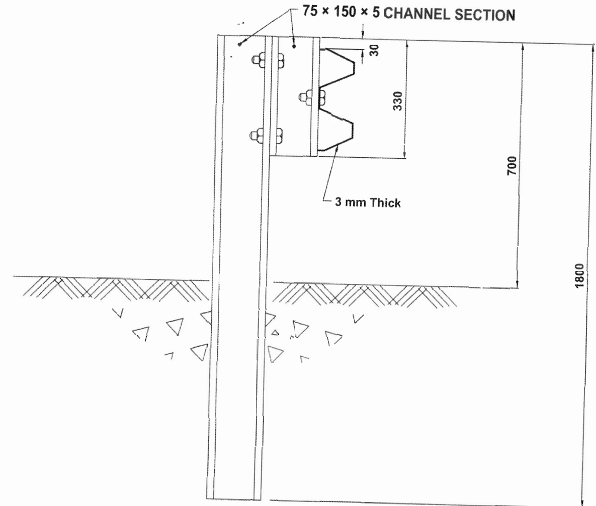
Fig. 9.2 Typical Details of "W" Beam Section
