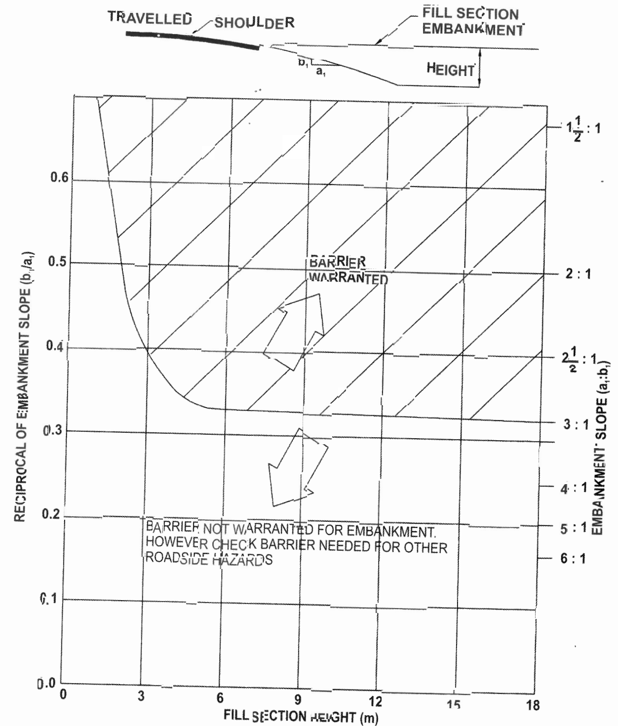
Fig. 9.1 Warrants for Roadside Barriers on Embankments
