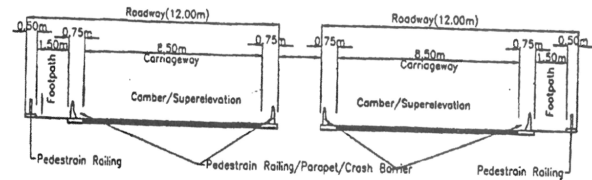
Fig. 7.2 Cross Section of Bridge at Deck Level - with Footpath 4-Lane Divided Highway
