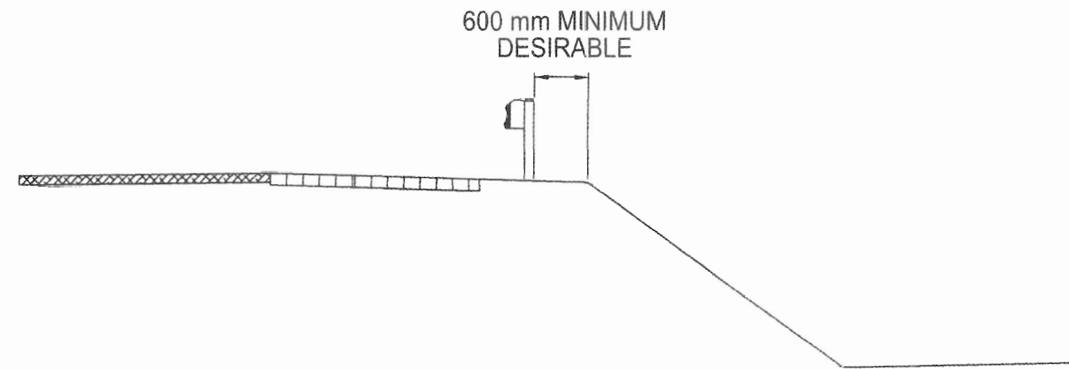
Fig. 9.4 Recommended Barrier Placement
