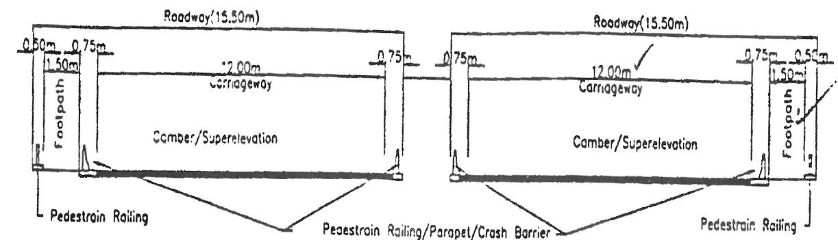
Fig. 7.3 Cross Section of Bridge at Deck Level - with Footpath 4-Lane Divided Highway (Both sides new Bridges for 6-Lane Standards)
