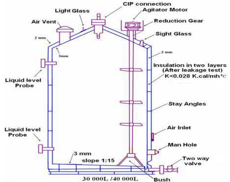
Fig. Vertical milk storage tank
