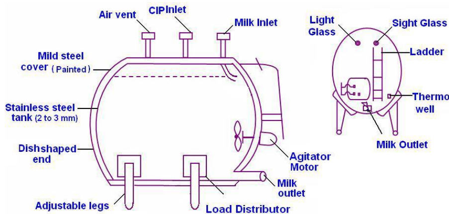
Fig. Horizontal milk storage tank
