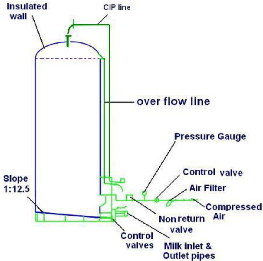
Fig. Milk silo tank
