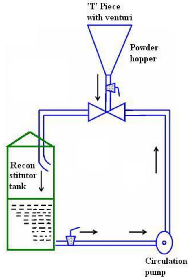
Fig. Reconstitution with funnel venturi system
