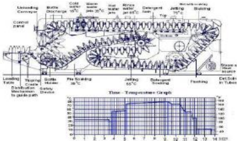
Fig. Bottle washers
