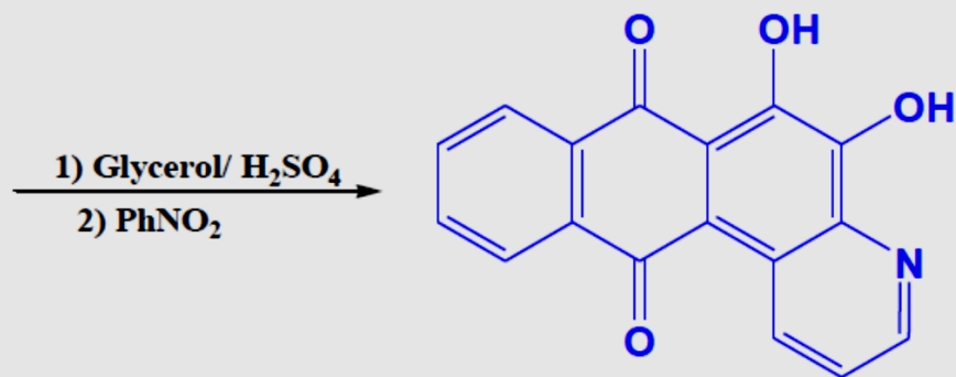
Alizarine Blue
