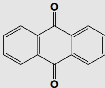
Anthraquinone
