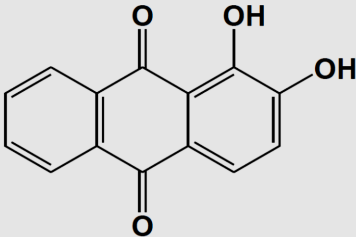
1,2-dihydroxyanthraquinone Alizarine
