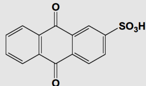
9,10-anthraquinone-2-sulfonic acid
