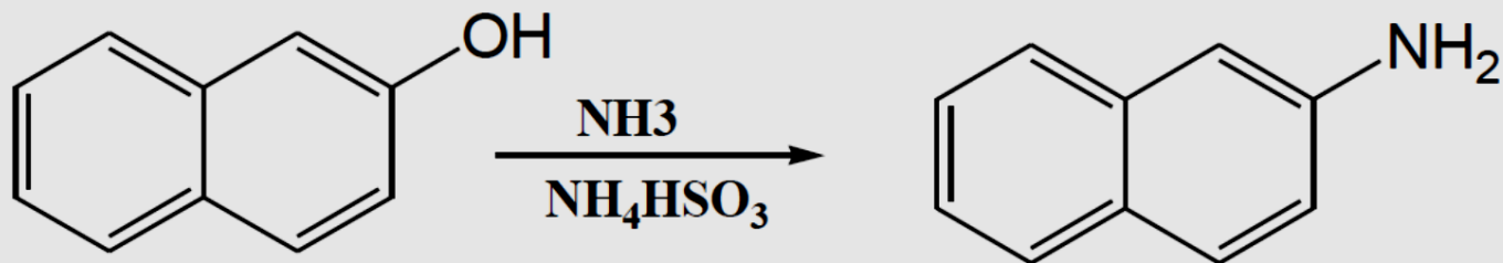
β- Naphthol
