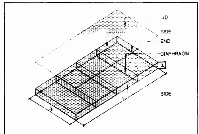
Fig. 2 Revet Mattress
