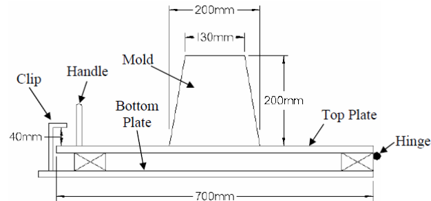
Figure 5: Flow table and cone
