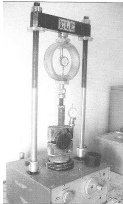
Stability Testing
