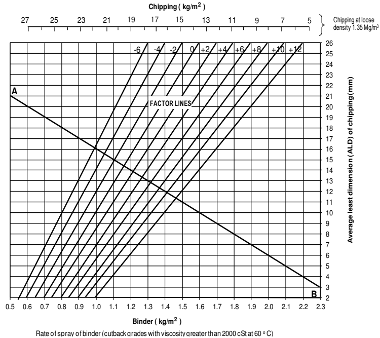
Figure 8: Bitumen and Chipping application rates
