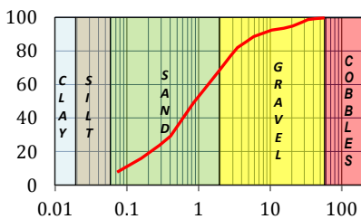
Particle Classification
