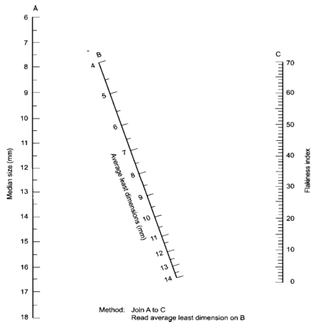
Figure 7: ALD chart
