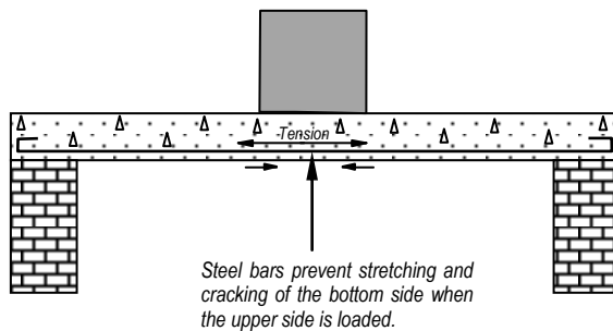
Figure 2: Tension in a concrete member with end support.
