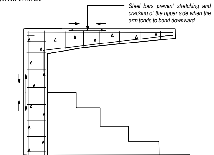
Figure 3: Tension in a concrete member with one end support.
