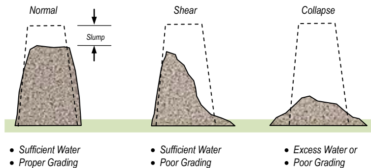
Figure 4: Common types of Slump
