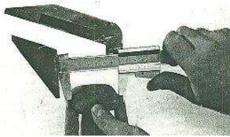
ALD measurement
