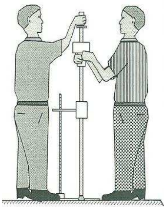
DCP Test
