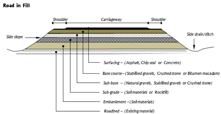
Figure 6: Typical cross-section of a road
