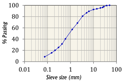
Grading Curve
