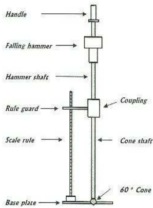
DCP Instrument
