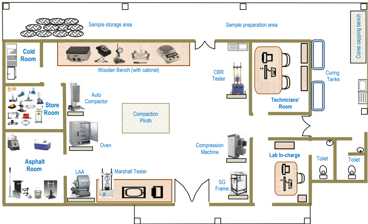
Figure 1: Typical laboratory arrangement
