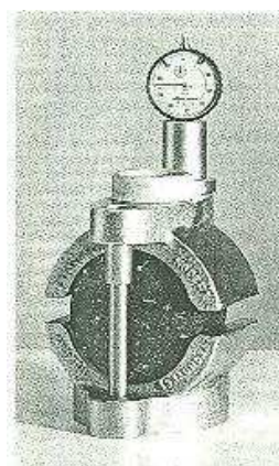
Crushing head and Flow gauge
