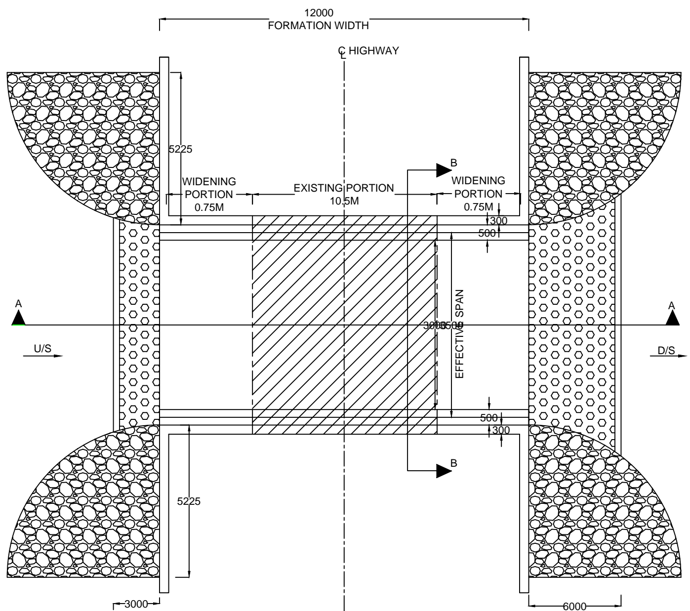
RCC SLAB CULVERT OF SPAN 3.5M & HEIGHT 3.5 M
