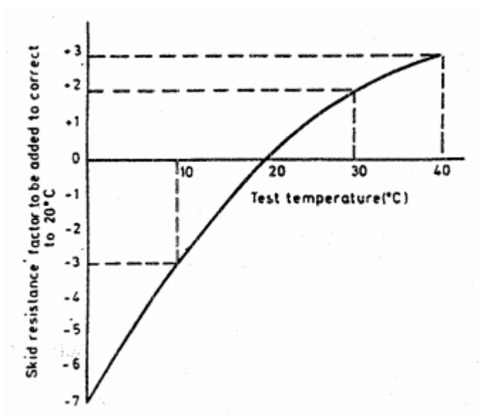
FIG. 2 SKID RESISTANCE/ TEMPERATURE CORRECTION RELATIONSHIP (TRRL, 1969)
