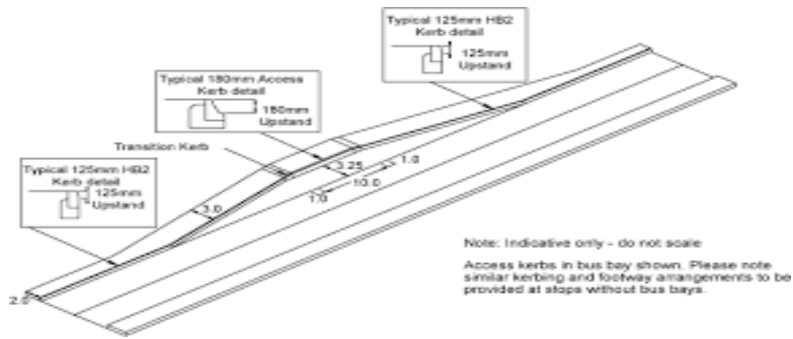
FIG.12 BUS-BAY PROVISION
