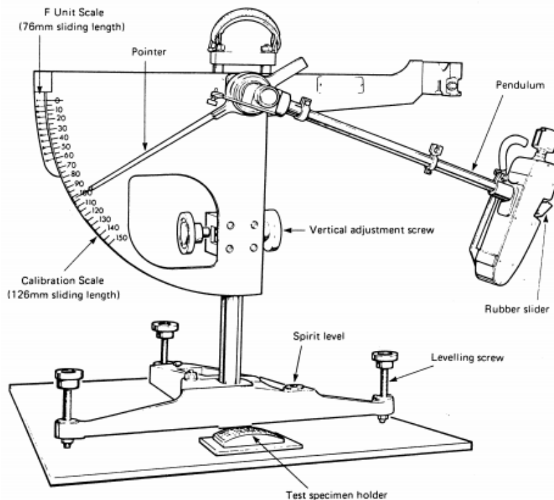
FIG.1 PENDULUM SKID RESISTANCE TESTER (BSI, 1990)
