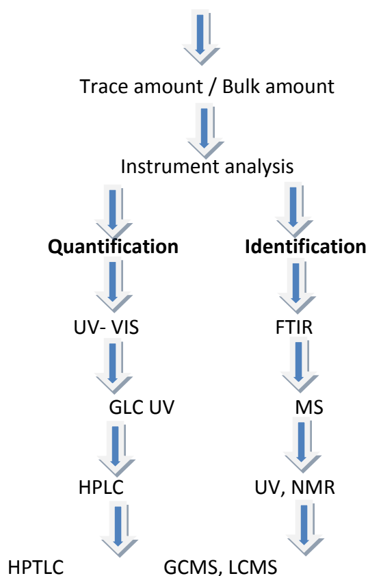
Figure 2: It shows a schematic diagram of possible steps for identification of novel drugs Crude Extract (Mixture of compounds) From TLC
