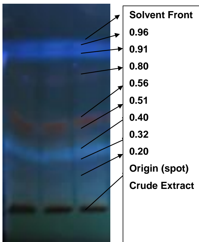
Figure 3: It shows various bands of secondary metabolites separated on TLC by using solvent system chloroform: ethyl acetate: benzene: glacial acetic acid (25: 15: 2: 10), Rf values of all bands are marked with solvent front and sample spot.
