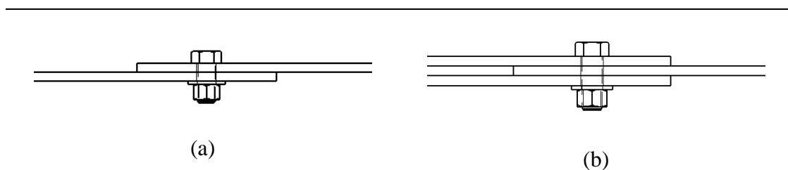
Figure 13 (a) Single shear (b) Double shear
