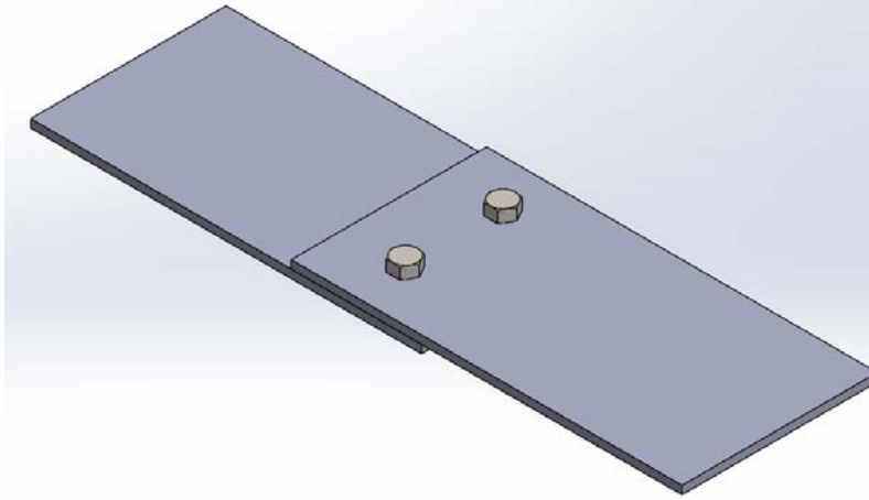
Figure 10 Bolted lap joint
