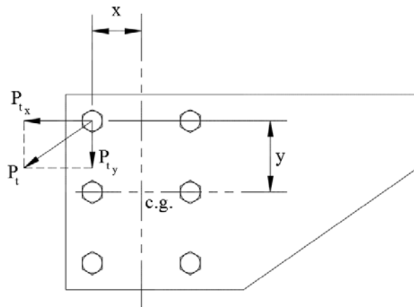
Figure 25 Development of torsional loading per bolt
