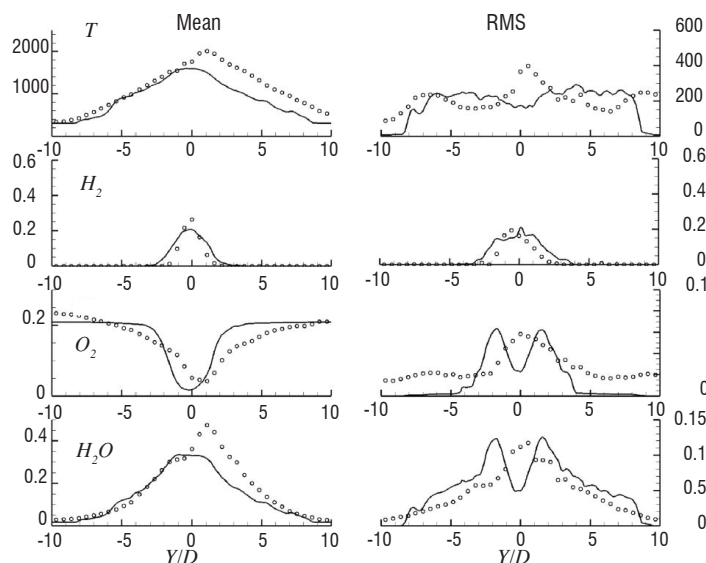
Figure 15 - Mean and RMS profiles of the temperature and main species mole fractions at X/D = 32.3
