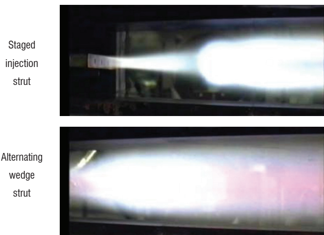
Figure 27 - Spontaneous emission visualization for the staged injection strut (top) and the alternating wedge strut (bottom)
