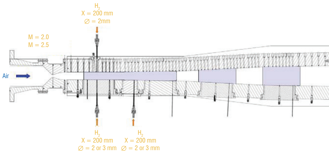
Figure 31 - Side view of the combustor equipped with wall hydrogen injectors
