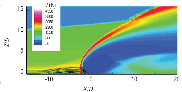
Figure 19 - R1294 (mean flow). Temperatures in the vicinity of the injection. Streamlines in the upstream boundary layer.
