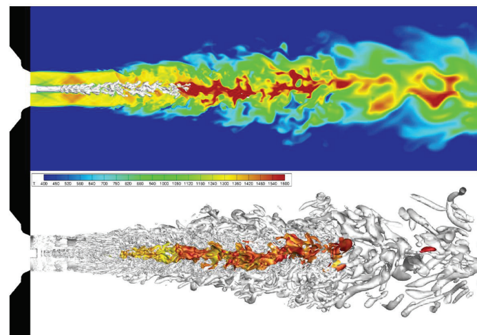
Figure 10 - Flame structure – Instantaneous field of temperature and H_2 mass fraction iso-surface [0.05] (top) - Iso-surfaces of Q-criterion [ 1 \times 10^9 ( s^{-2} )] and OH mass fraction [0.01] colored by temperature (bottom)
