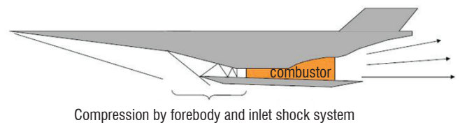
Figure 43 - Typical scramjet powered hypersonic vehicle layout
