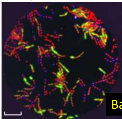
Figure 2.13 Fluorescent Dyes and Tags. (a) Dyes that cause live cells to fluoresce green and dead ones red; (b) Auramine is used to stain Mycobacterium species in a modification of the acid-fast technique; (c) Fluorescent antibodies tag specific molecules. In this case, the antibody binds to a molecule that is unique to Streptococcus pyogenes .
