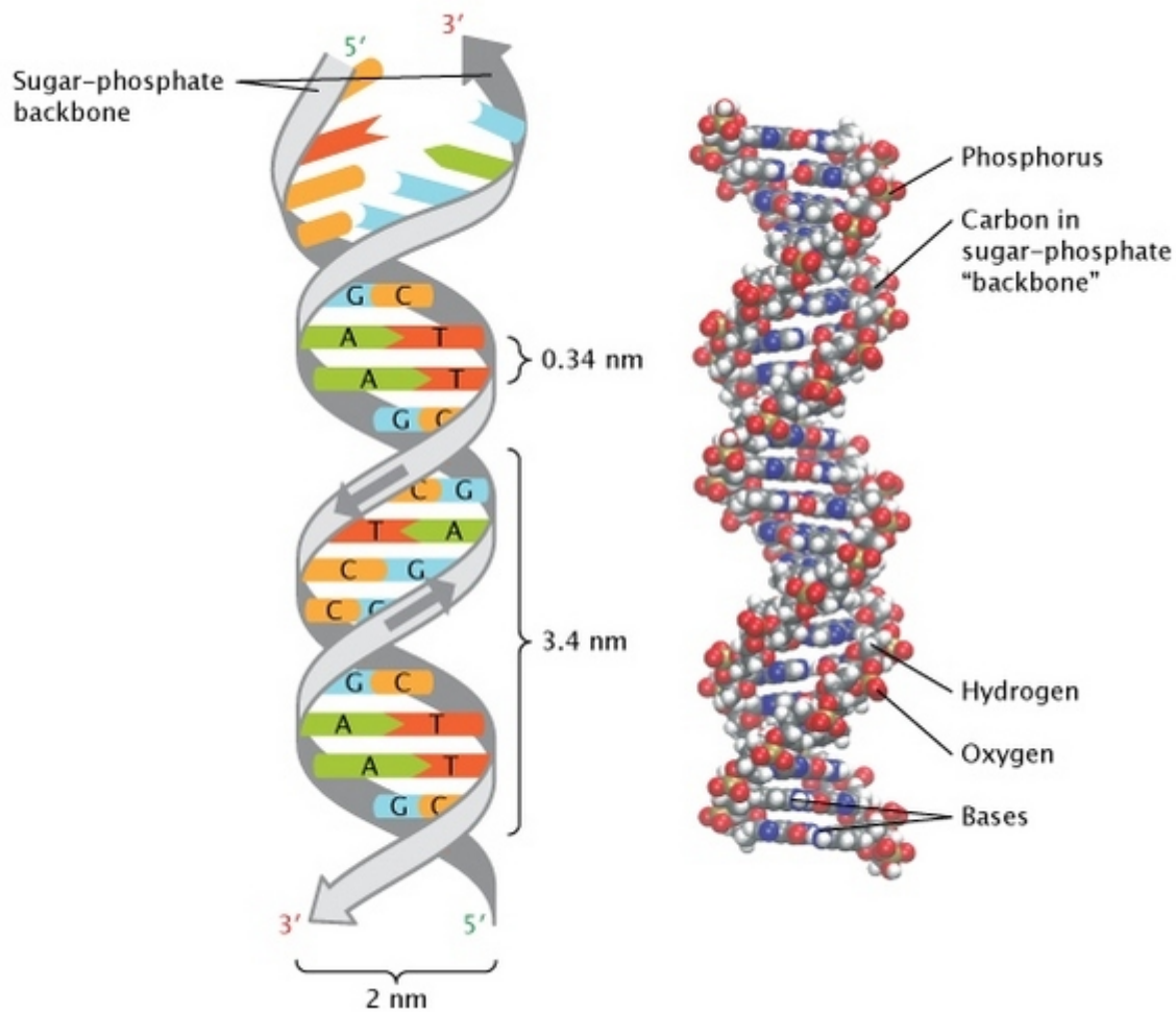
Figure 3: The double-helical structure of DNA.
