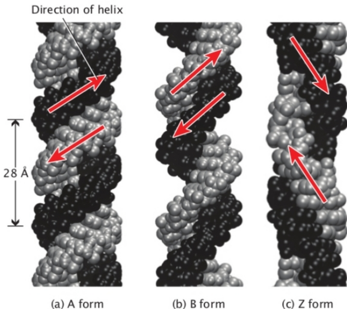
Figure 5: Three different conformations of the DNA double helix.
