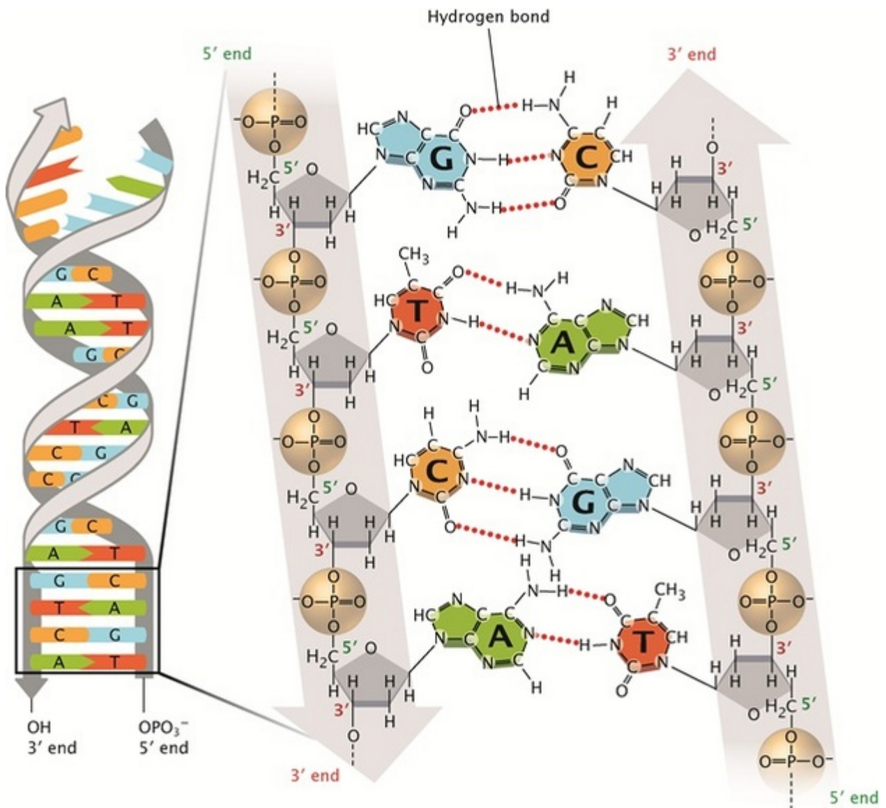
Figure 4: Base pairing in DNA.
