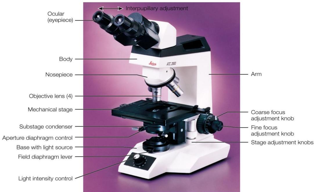
Fig : A compound Microscope.
