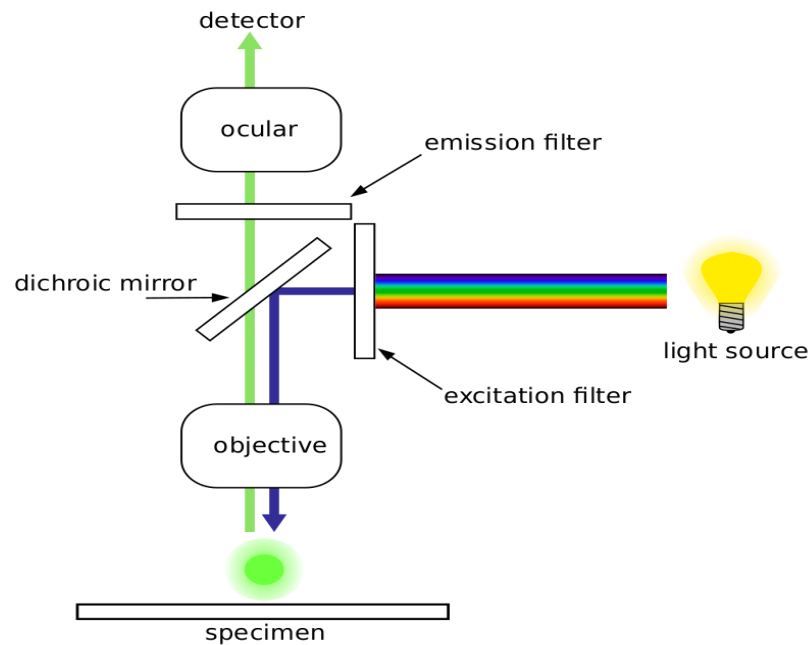
Fig: Working of Fluorescence Microscope
