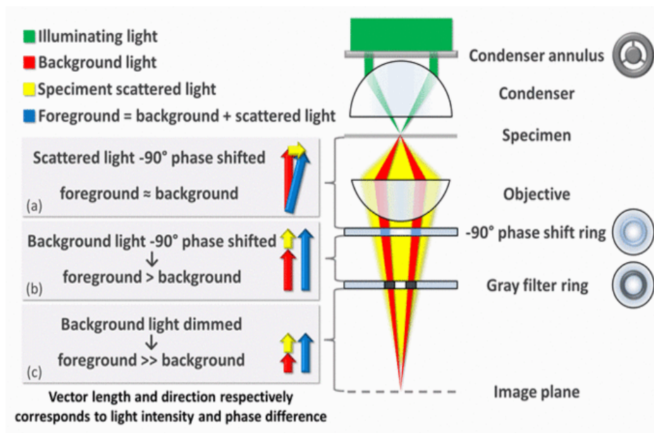
Fig: A Phase Contrast Microscope with working Principal.
