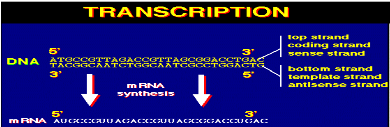
Fig :Transcription
