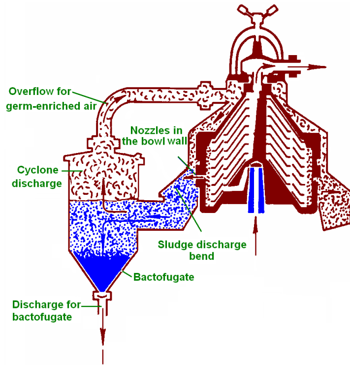
Fig. 21.1 Hermatic bactofuge
