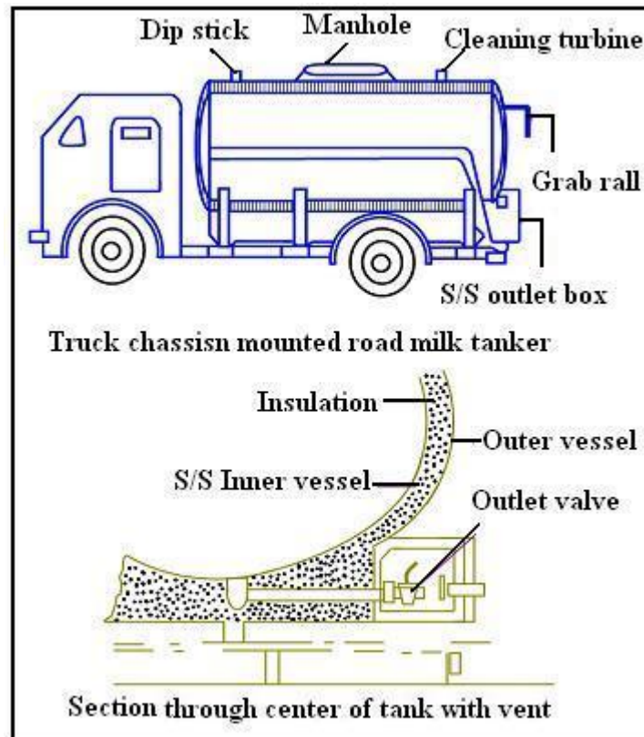
Fig. 9.1 Road tanker
