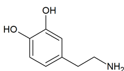
dopamine (neurotransmitter)
