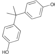
Figure 1: Bisphenol A
