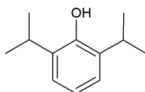
propofol (pharmaceutical)
