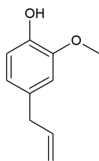
eugenol (perfume)
