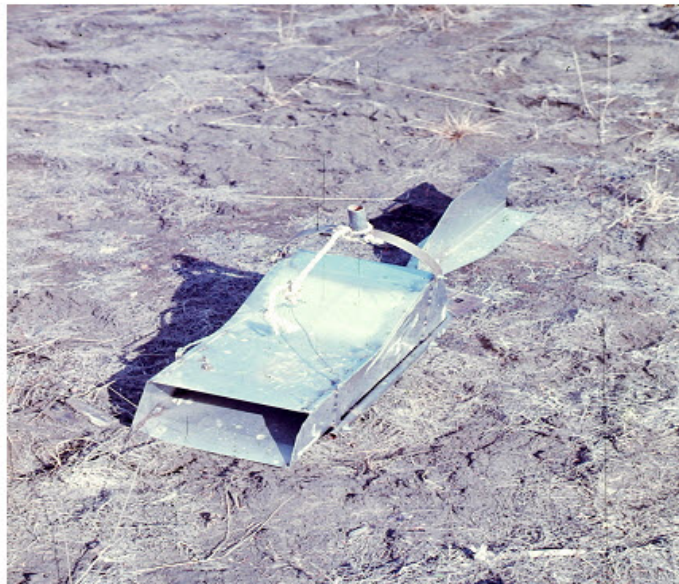
Fig. 20.1. A Commonly Used Type of Bed-load Sampler. (Source: http://www.sfu.ca/~hickin/RIVERS/Rivers4(Sediment transport).pdf )
