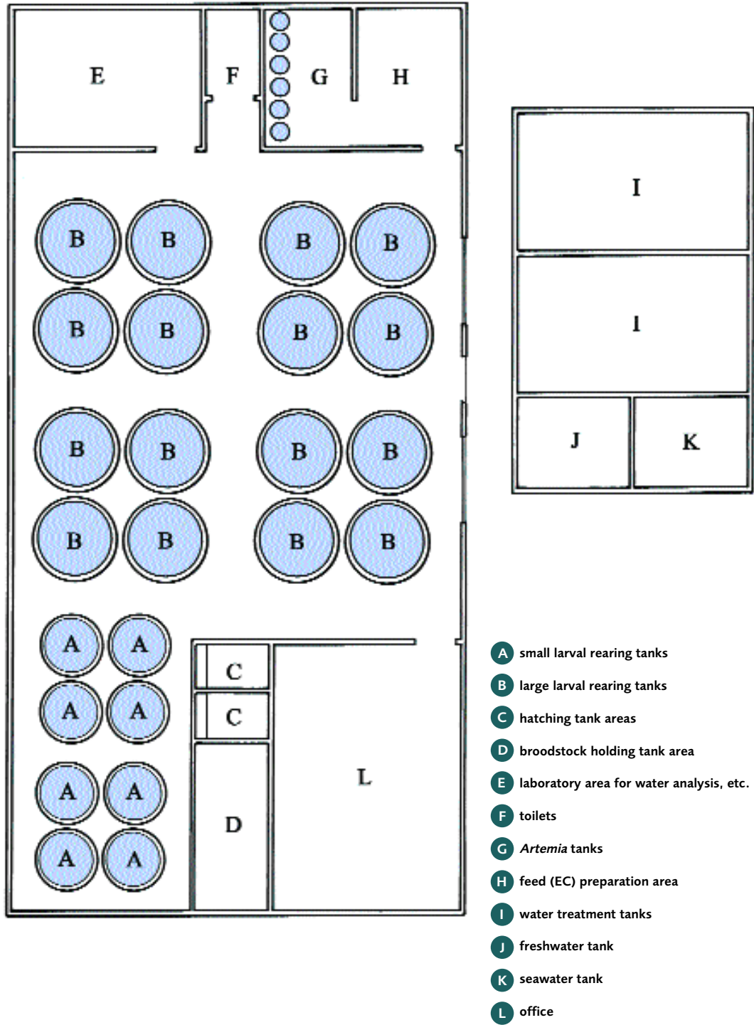
Hatchery layout is site specific; this is one example
