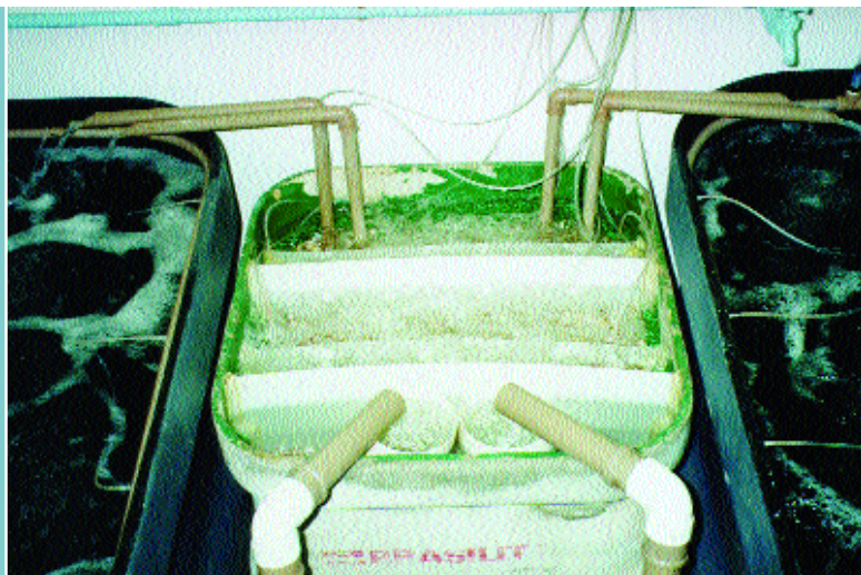
Figure 31 Close-up of a biological filter shared between two larval tanks in Brazil, showing the water entering the mechanical filters (foreground), from where it passes through the biological filter and exits back to the two tanks by means of simple airlift pumps
