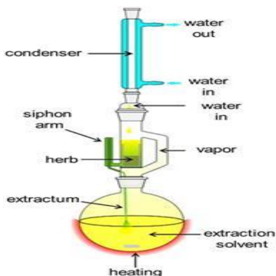
Fig 9.1: Soxhlet apparatus
