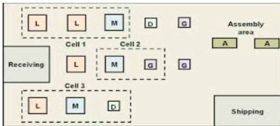
Fig. 5 Group layout or Cellular layout
