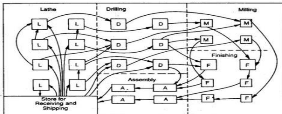
Fig. 1 Process layout
