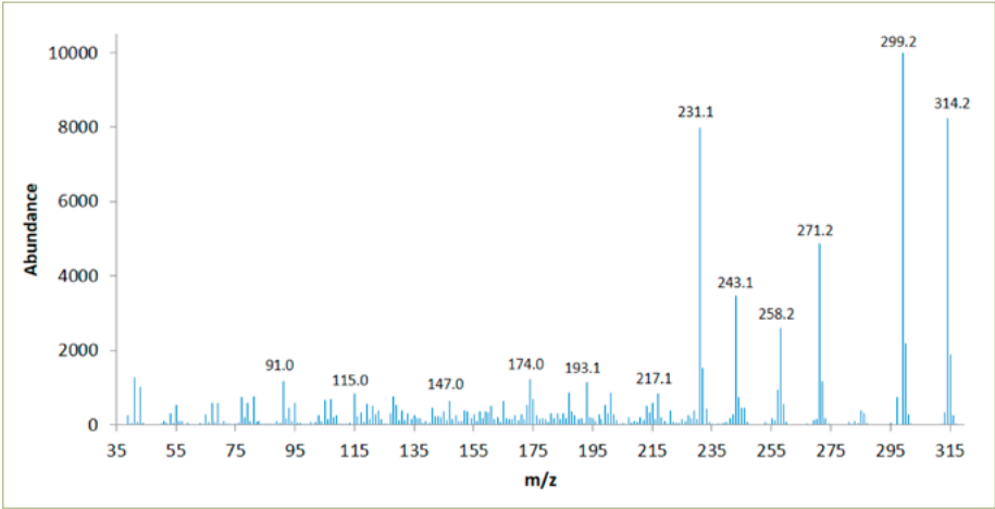
Figure XIV. GC-MS spectra of THC isomers
