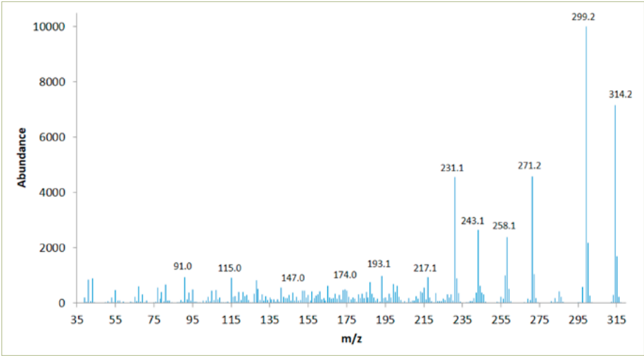
Mass Spectrum of (6aR,9R)- \Delta^{10} -THC
