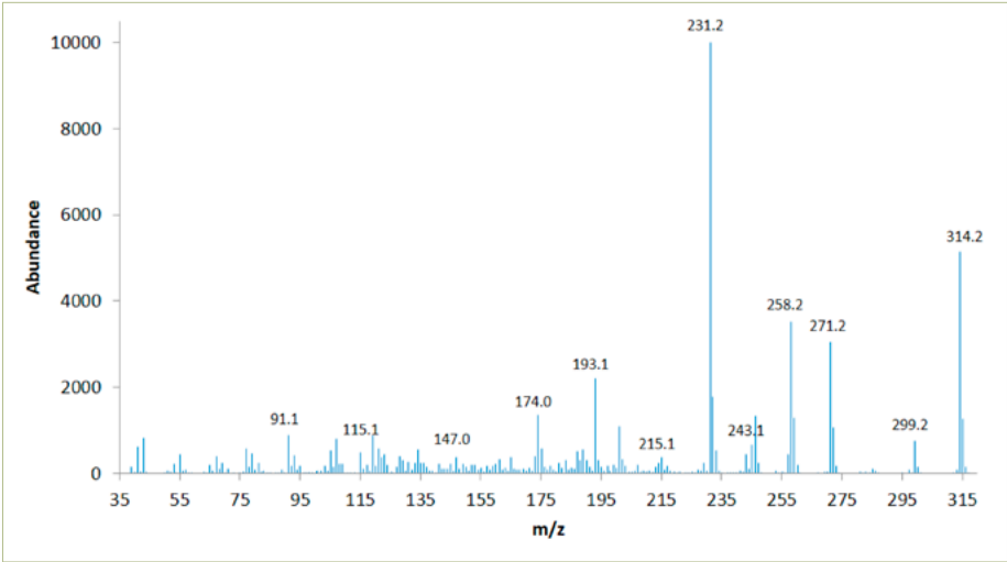
Mass Spectrum of (-)- \Delta^8 -THC
