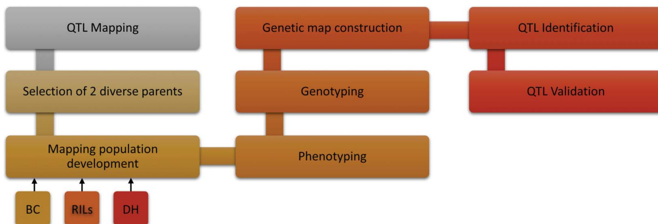
Figure 1. QTL mapping methodology.
