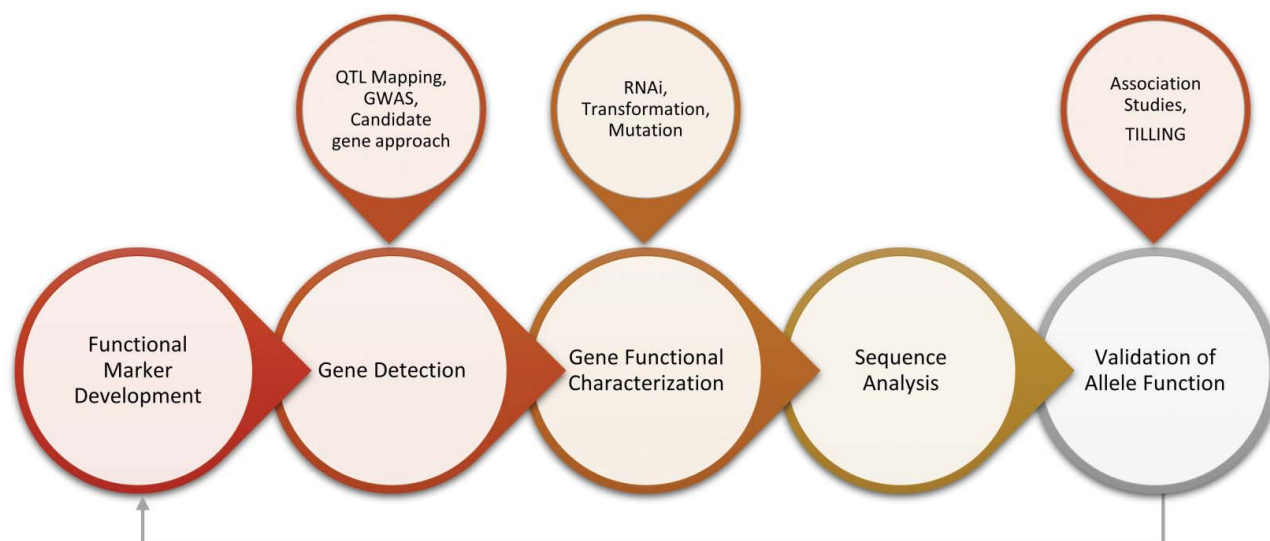
Figure 4. Important steps involves in the development of functional markers.
