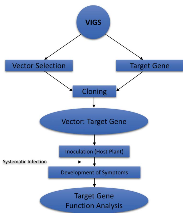
Figure 6. General methodology of VIGS.
