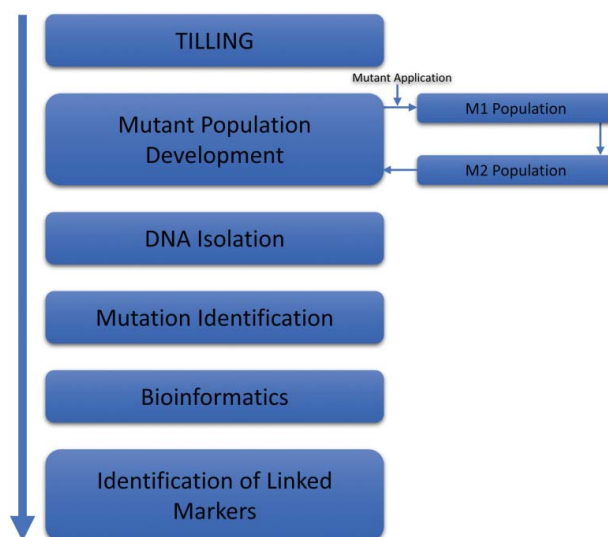
Figure 5. Important steps involved in TILLING.
