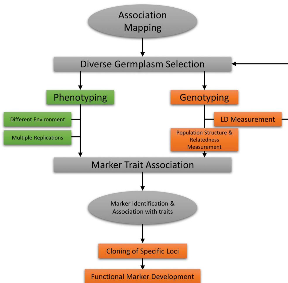
Figure 2. Methodology of association mapping.
