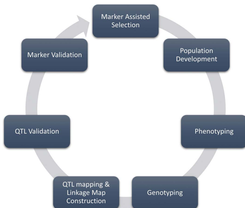
Figure 3. Some important steps involves in MAS.
