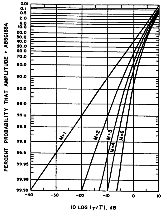
Fig. 11 Graph of probability distributions of SNR=\gamma threshold for M branch selection diversity. The term \Gamma represents the mean SNR on each branch
