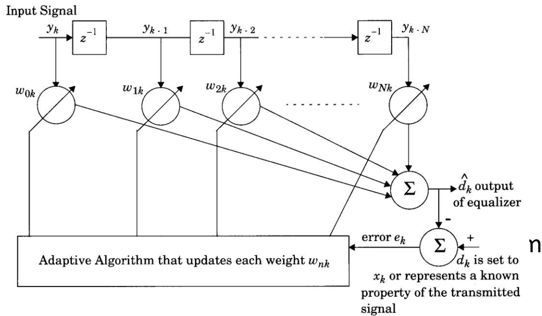
A basic linear equalizer during training.
