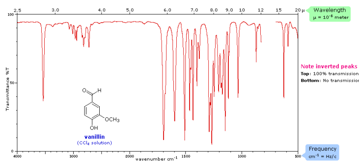
Figure 5.4.1: Infrared spectrum of vanillin. (CC BY-
