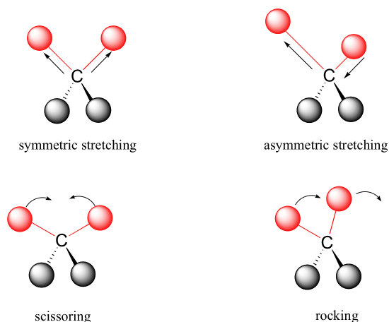
Figure 5.4.1: Types of vibrational modes. (CC BY-NC-SA; Layne A. Morsch via LibreTexts)
