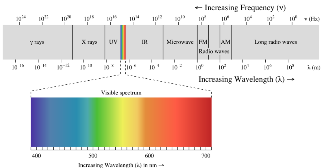
Figure 5.4.1: The electromagnetic spectrum. (CC BY-NC-SA; Brittany Stadler via LibreTexts)
