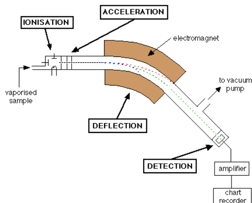
Figure 5.5.1: Basic diagram of a mass spectrometer. (CC BY-NC-SA; Jim Clark via LibreTexts)
