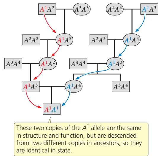
(b) Alleles identical by state
