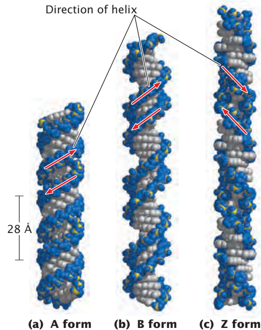
10.15 DNA can assume several different secondary structures.
