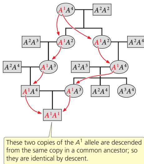
(a) Alleles identical by descent
