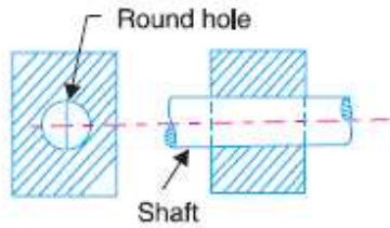
Fig: Shaft in a circular hole.
