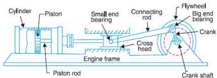
Fig: Reciprocating steam engine
