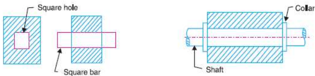
Fig: Square bar in a square hole. Fig: Shaft with collars in a circular hole.
