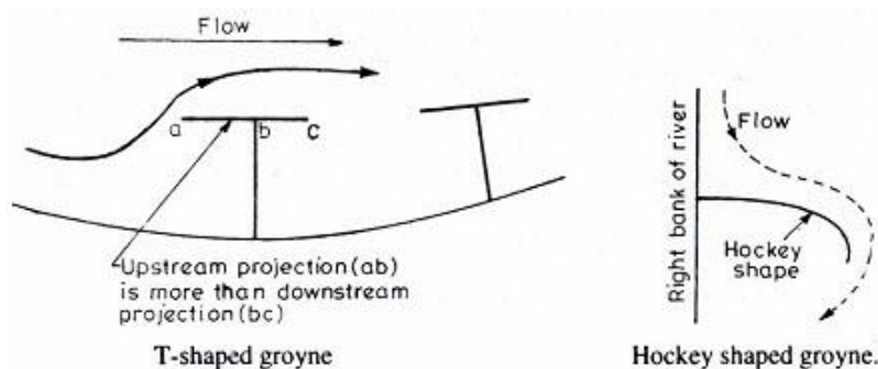
Fig. 13.7. 'T' Head and Hockey Stick Shaped Head Groynes.
