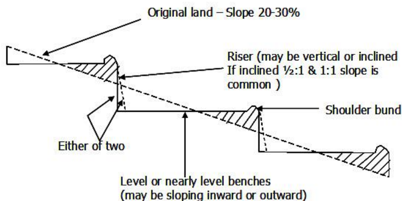
Fig. 5.2. Bench terrace and its different components.
