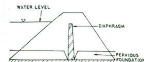
Fig. 11.4. Diaphragm Earthen Dam.
