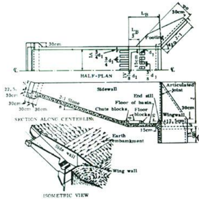
Fig. 10.3. Outline Section of Chute Spillway Provided with SAF Stilling Basin.
