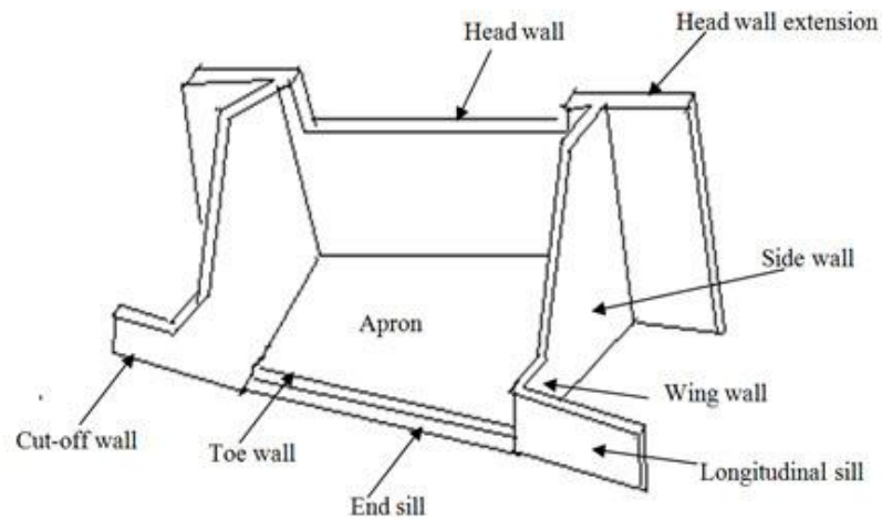
Fig. 8.1. Drop spillway.
