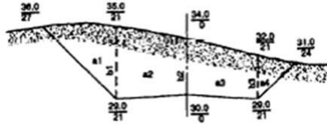
Fig. 24.6. Cross Section Cut Showing Distances and Elevations
