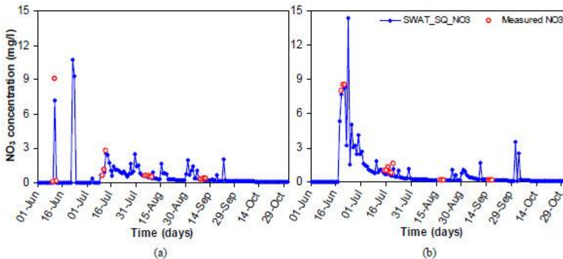
Fig. 32.9. Measured and SWAT Simulated NPS \text{NO}_3\text{-N} concentration at the Watershed Outlet in 2000 (a) and in 2001 (b). (Source: Mishra et al., 2009)
