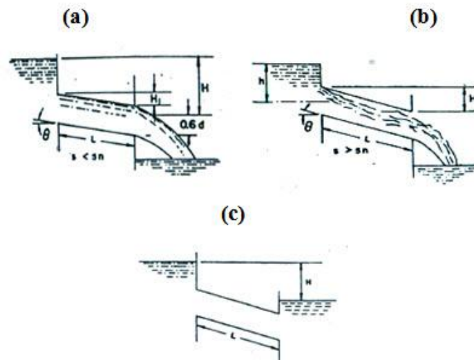
Fig. 9.3. Different flow conditions (a) Full free outfall pipe flow; (b) Part full: free outfall orifice flow; (c) Full: outfall submerged pipe flow in drop inlet spillway.
